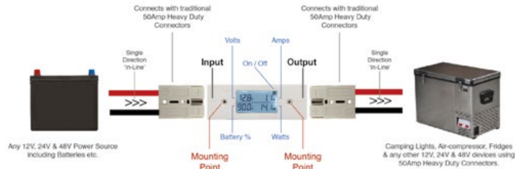
One of the many possible configurations of the KT 125A, 100V In-line Power Meter and your devices.
