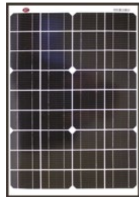
KT SOLAR 20W, 12V MONOCRYSTALLINE SINGLE CELL SOLAR PANEL
