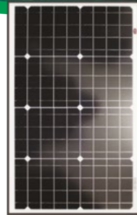
KT SOLAR 40W, 12V MONOCRYSTALLINE SINGLE CELL SOLAR PANEL
